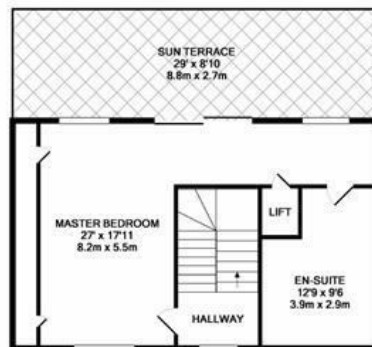
2ND FLOOR
